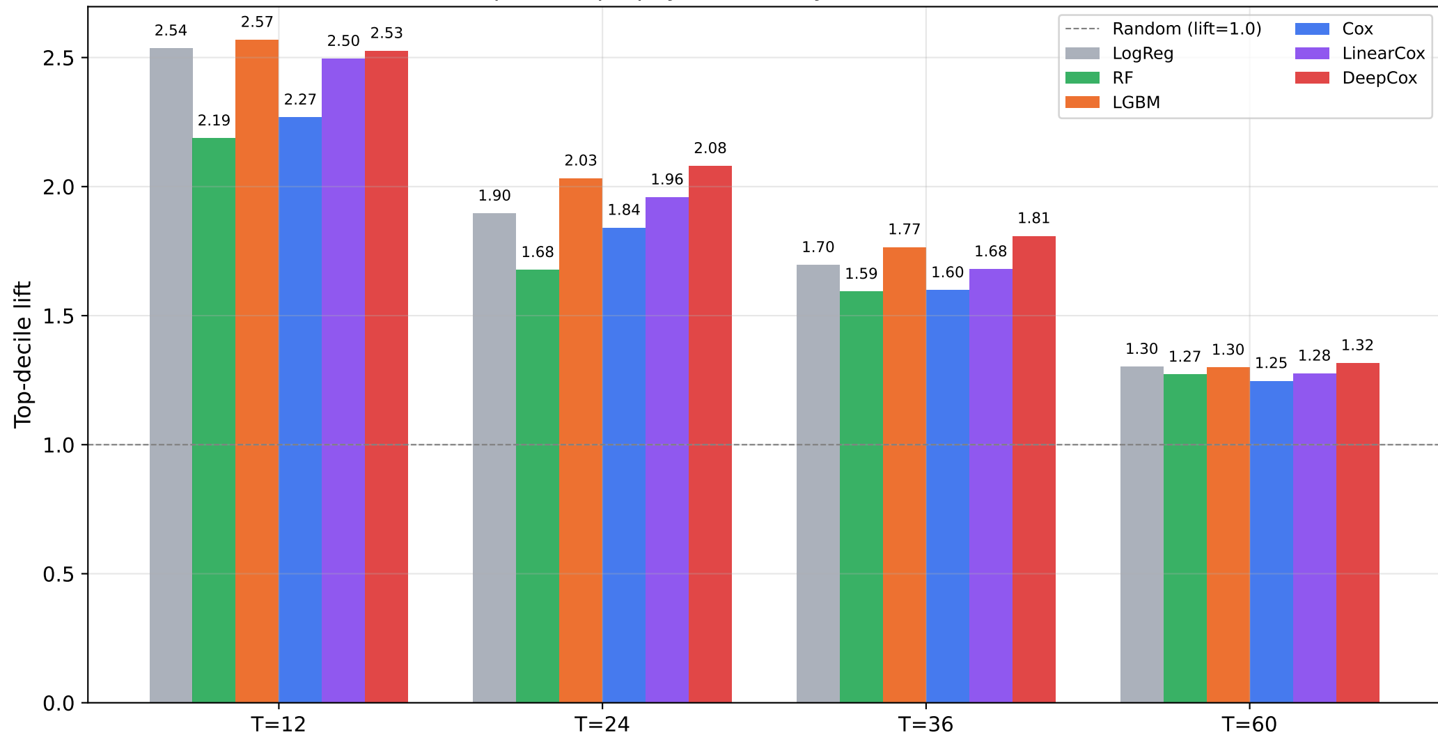
Top-decile prepayment lift, by horizon and model
